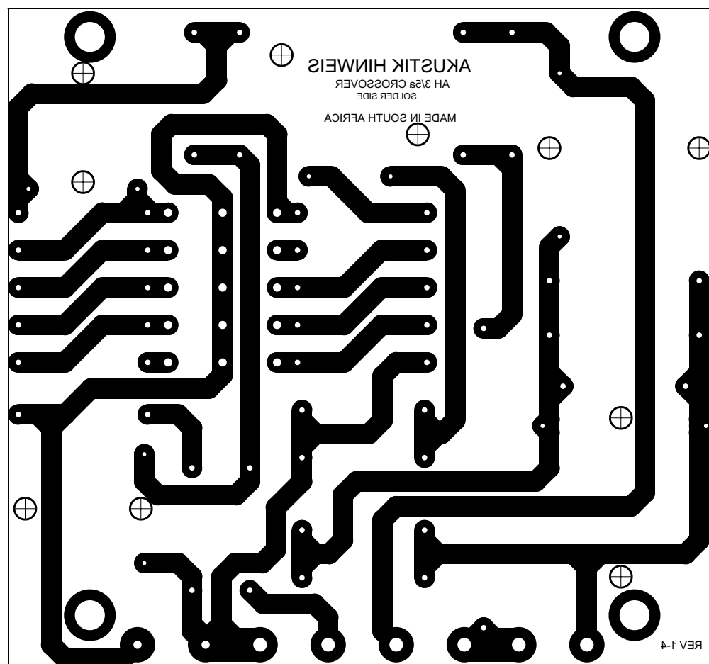
Board Track Layout (Viewed through the board)
